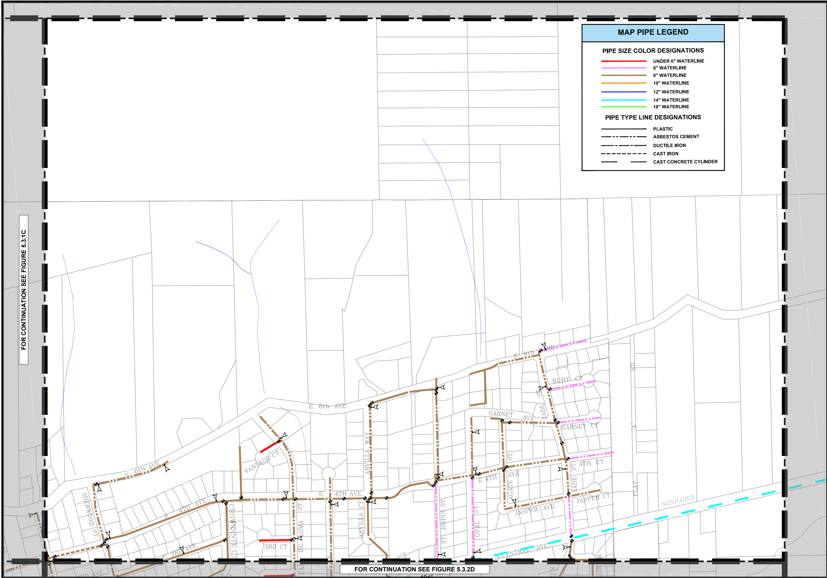
SUTHERLIN WATER MASTER PLAN EXISTING WATER SYSTEM
