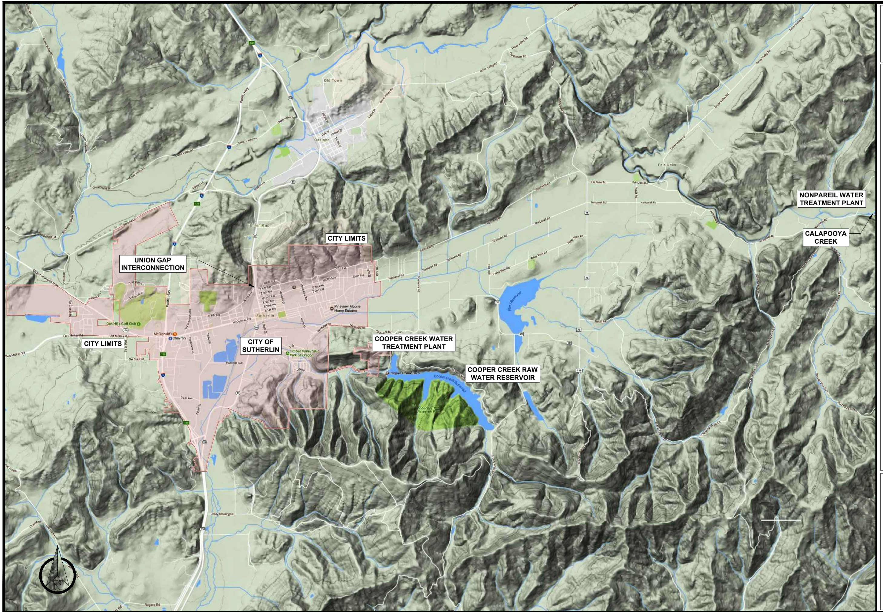
SUTHERLIN WATER MASTER PLAN
