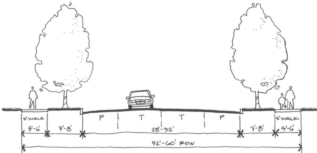
Figure 7-20. Local Residential Street– Parking Both Sides
