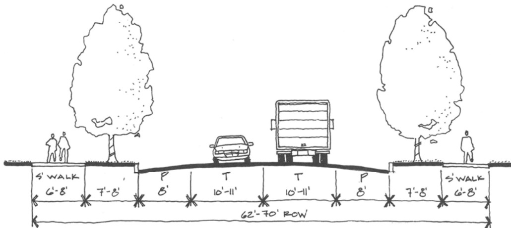
Figure 7-15. Commercial / Industrial Collector – Parking Both Sides
