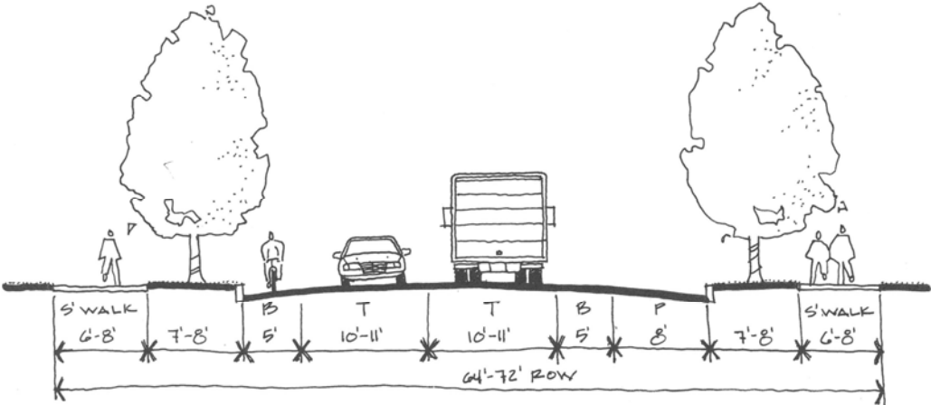
Figure 7-16. Commercial / Industrial Collector – Parking One Side
