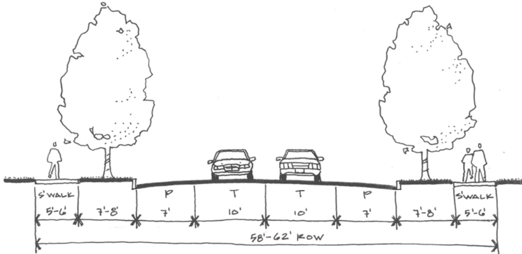
Figure 7-18. Residential Collector
