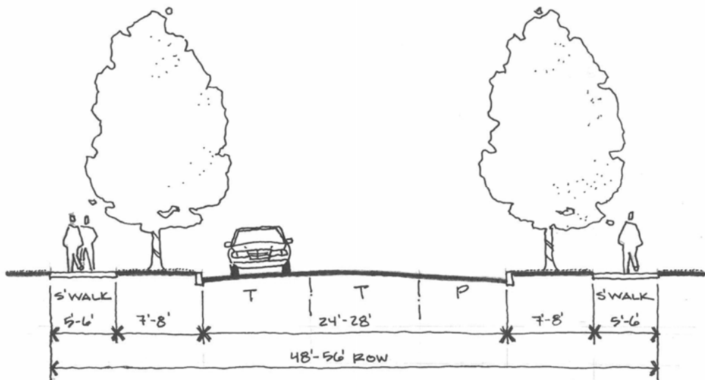
Figure 7-19. Local Residential Street – Parking One Side
