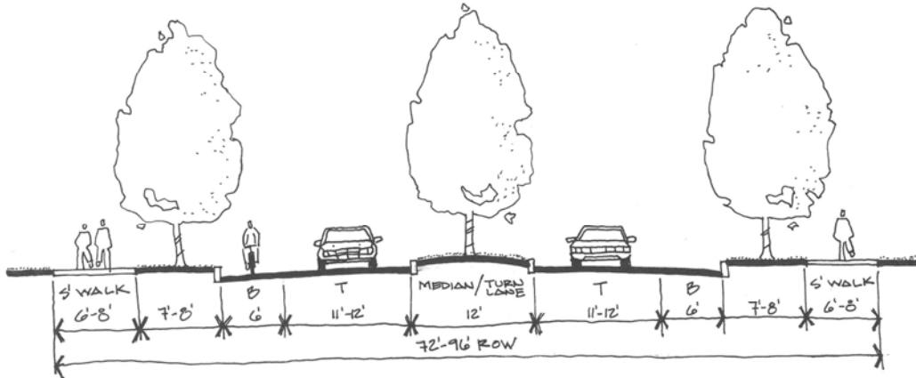
Figure 7-11. Three-Lane Arterial
