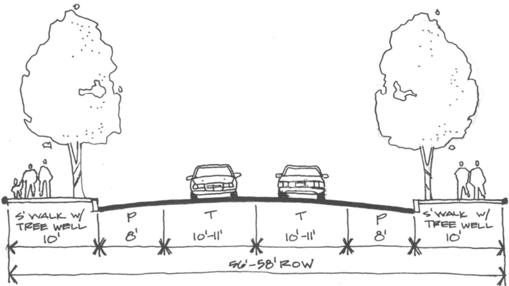
Figure 7-17. Commercial / Mixed-Use Collector – Parking Both Sides
