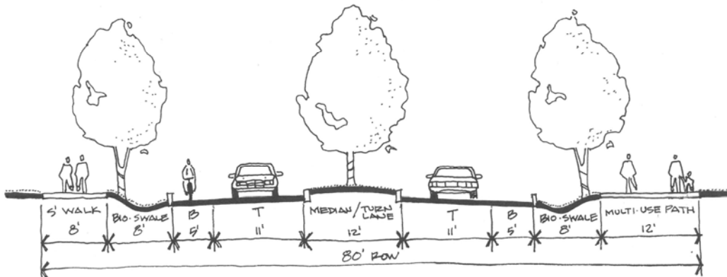
Figure 7-13. Parkway
