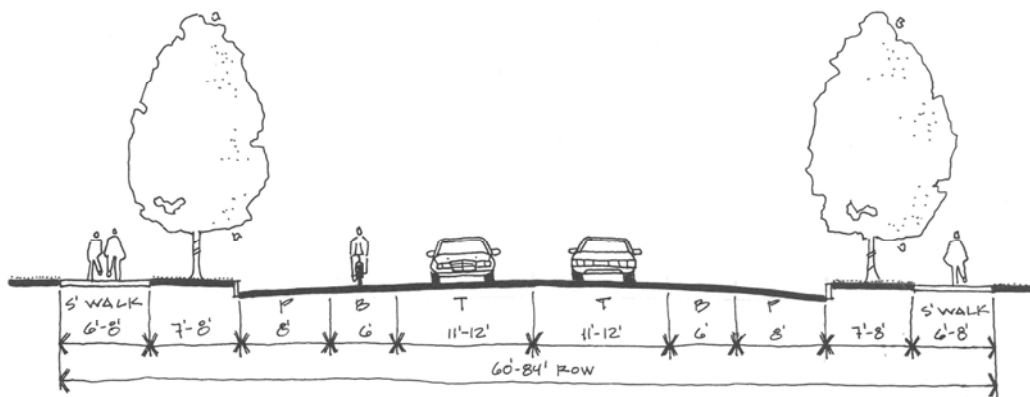
Figure 7-10. Two-Lane Arterial – Parking Both Sides
