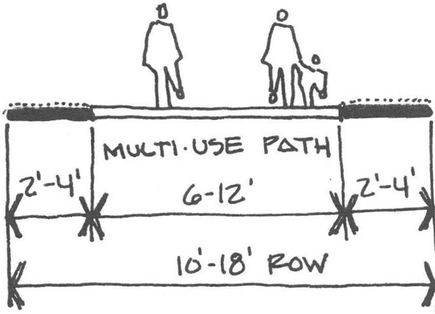
Figure 9-2. Multi-Use Path Cross Section
