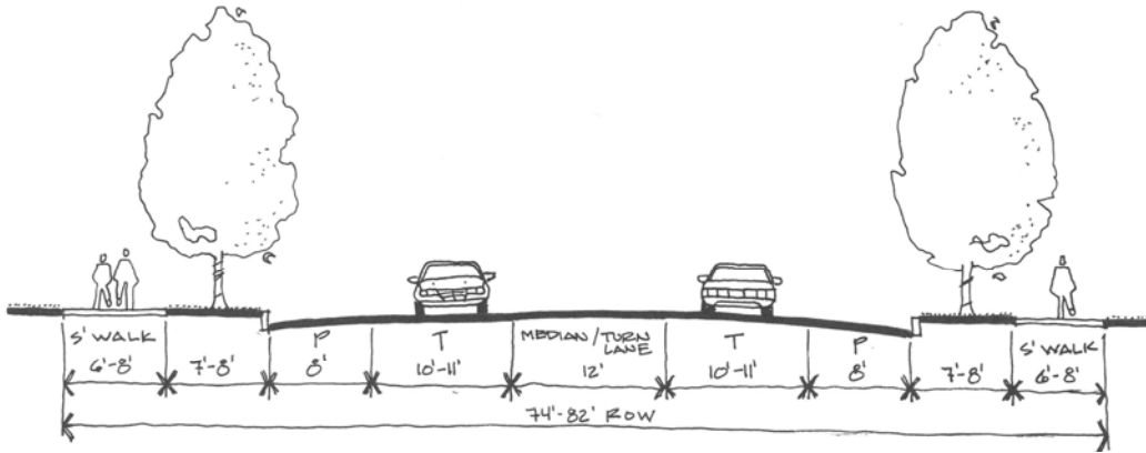
Figure 7-14. Three-Lane Collector – Parking Both Sides
