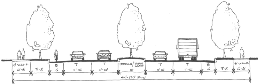
Figure 7-12. Five-Lane Arterial
