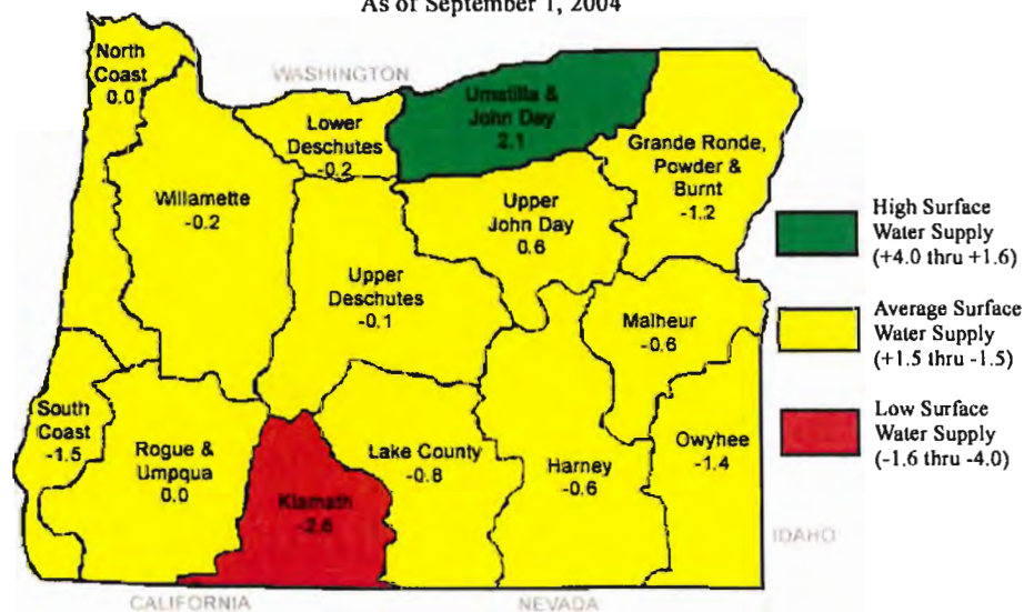
FIGURE 10.4.2 ILLUSTRATION OF SURFACE WATER SUPPLY INDEX (SWSI)
