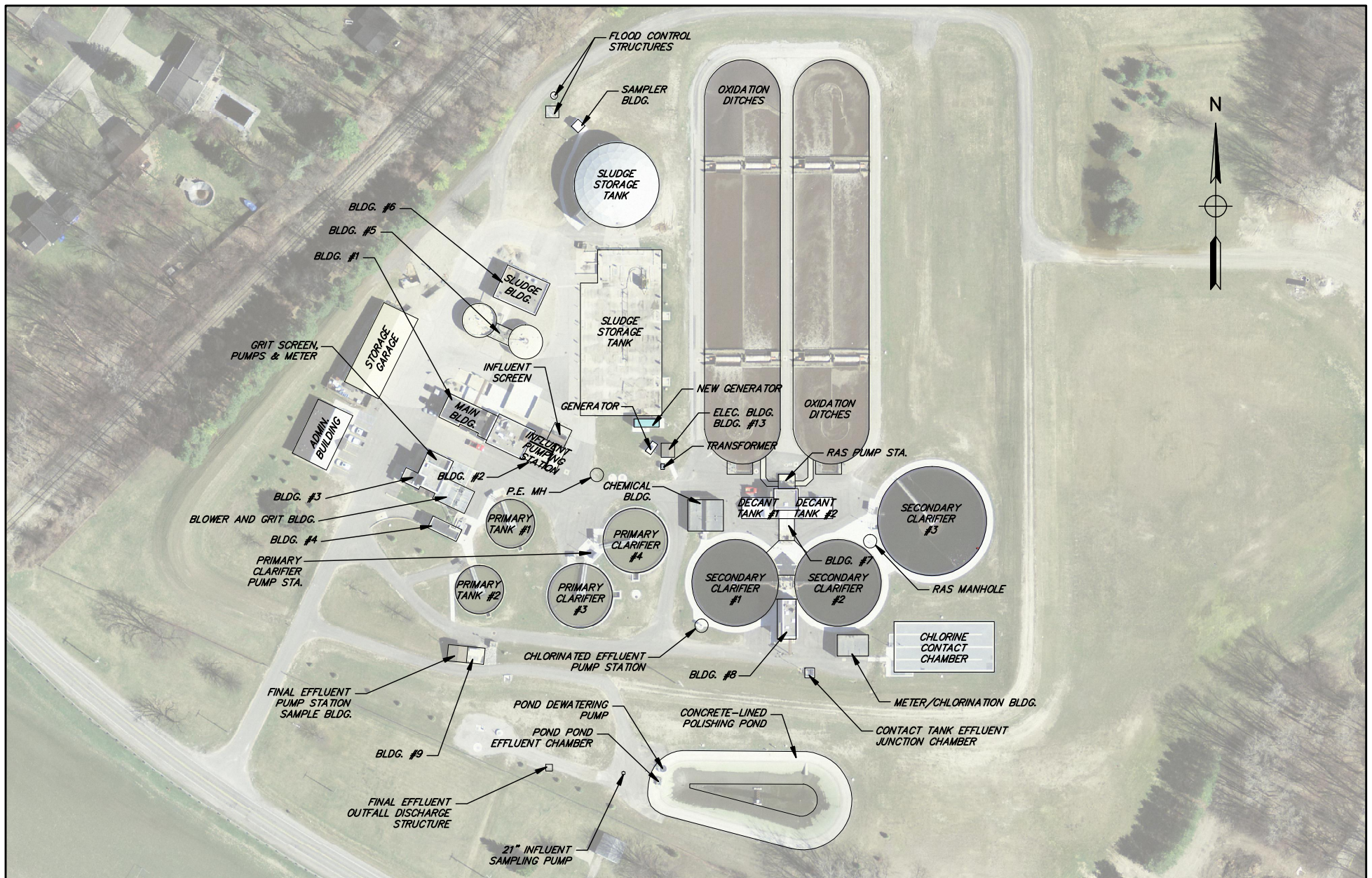
SAGINAW CHARTER TOWNSHIP WASTEWATER TREATMENT PLANT SITE LAYOUT
