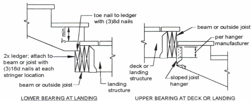
Figure 28 STRINGER BEARING
