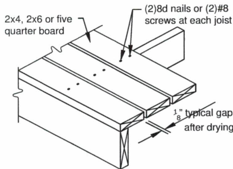
Figure 22 TYPICAL DECKING
