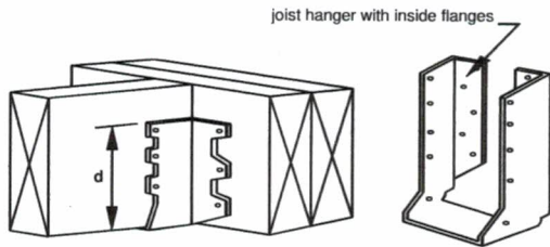
Figure 9 JOIST HANGERS
