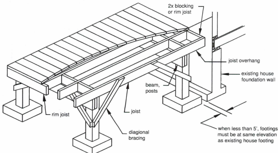
Figure 17 FREE-STANDING DECK
