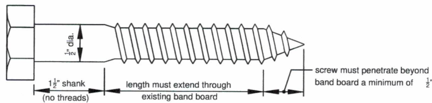
Figure 16 LAG SCREW
