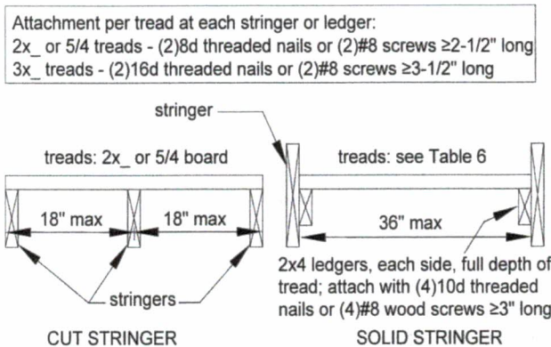
Figure 31 STAIRWAY TREADS
