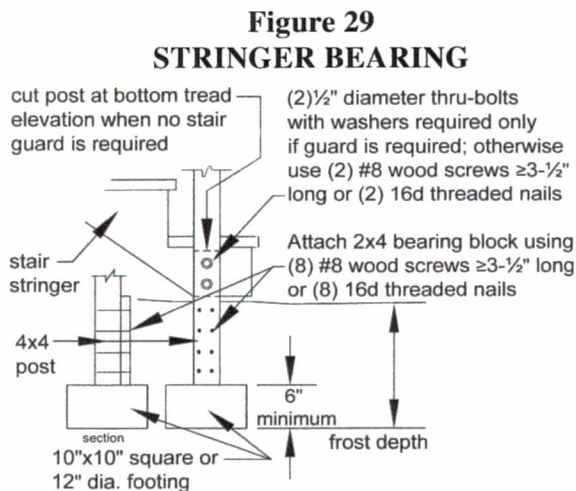
LOWER BEARING AT FOOTING
