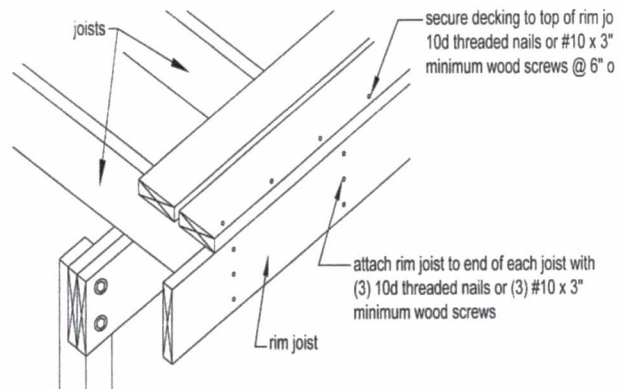
Figure 23 RIM JOIST CONNECTION
