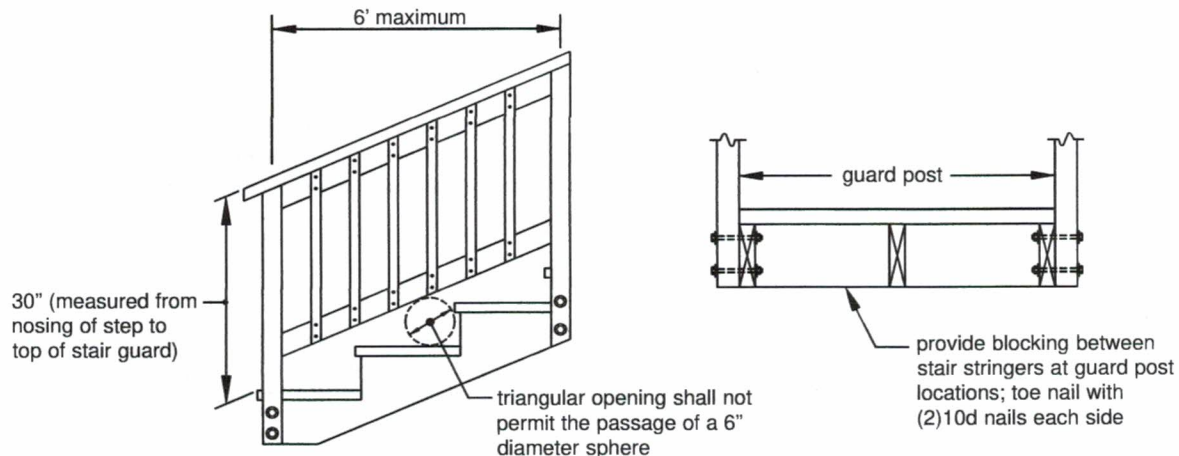
Figure 32 STAIR GUARDS
