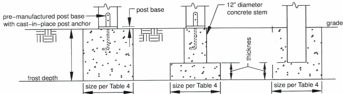
Figure 1 FOOTINGS
