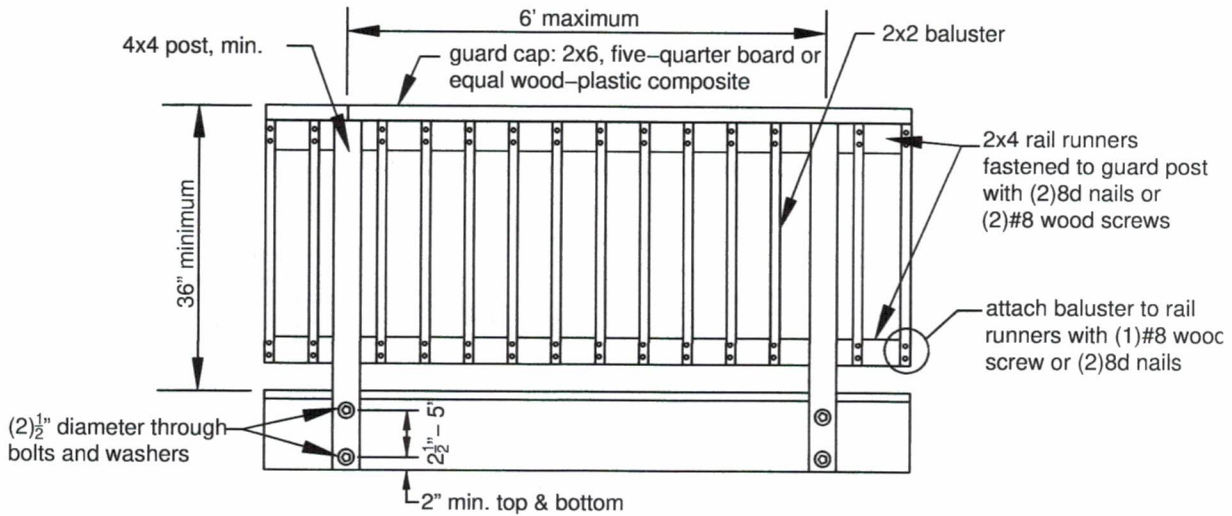
Figure 24 GUARDS
