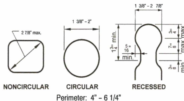
Figure 34 HANDRAIL GRASPABILITY
