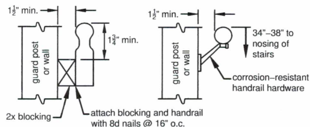
Figure 34 HANDRAIL GRASPABILITY
