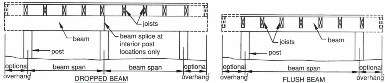
Figure 3 BEAM TYPES
