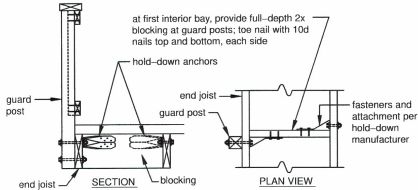
Figure 26 GUARD POST TO RIM JOIST
