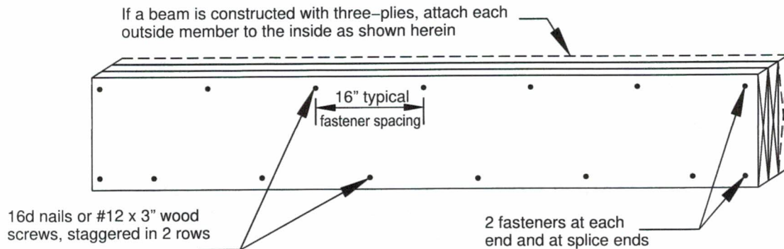
Figure 4 BEAM ASSEMBLY
