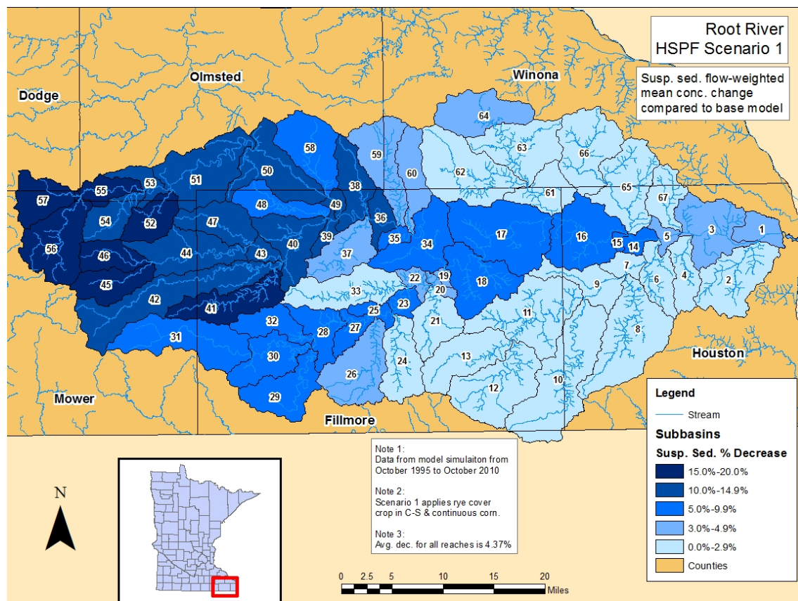
Figure 3: Suspended Sediment Decrease For Scenario 1
