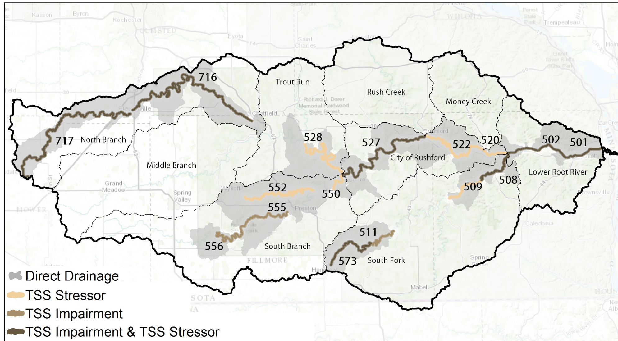
Figure 19. Sediment prioritization based on where suspended sediment (TSS) and aquatic life use impairments based on TSS occur in the Root River watershed.
