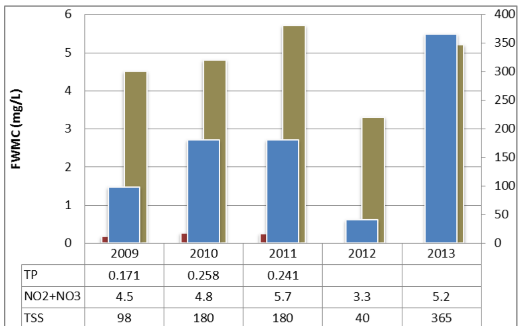
Figure 7. Watershed Pollutant Load Monitoring Network results reported in flow-weighted mean concentration (FWMC) for years 2009-2013. Blue bars indicate TSS; brown bars indicate NO3+NO2; red bars indicate phosphorus. Note: total phosphorus data is not available for 2012 or 2013.
