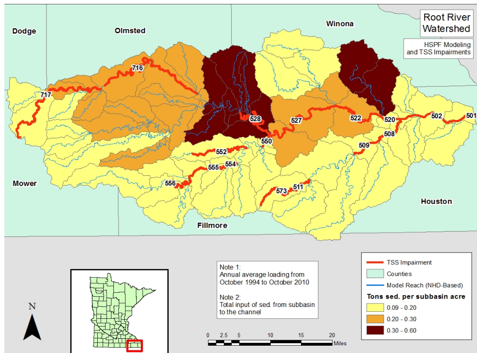
Figure 1: HSPF sediment loading and TSS impairments
