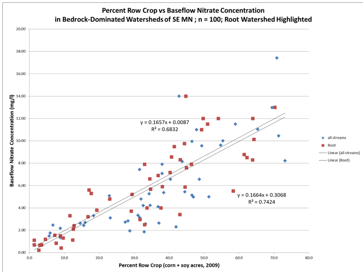
Figure 14. Baseflow nitrate and row crop acres regression (Watkins et al 2013). Root River data points are shown in red.
