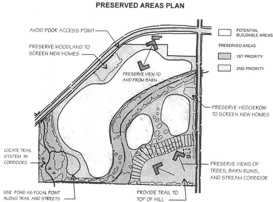
Figure 4 CONSERVATION SUBDIVISION DESIGN: STEP 2
